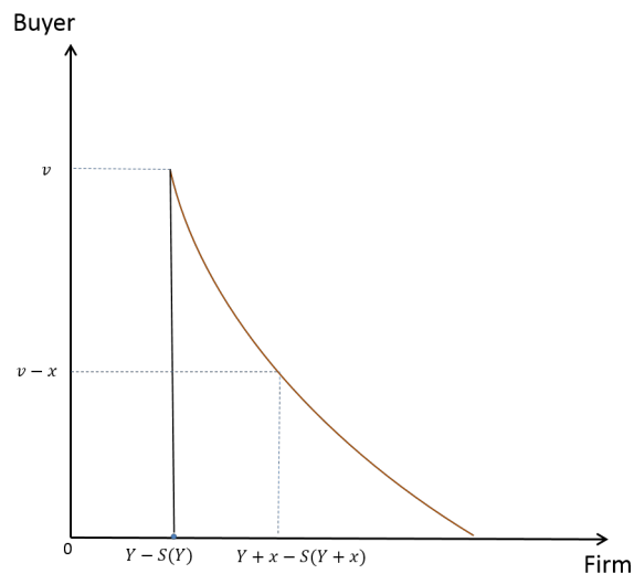
Figure 4: Payoff frontier B_j(S, Y)
