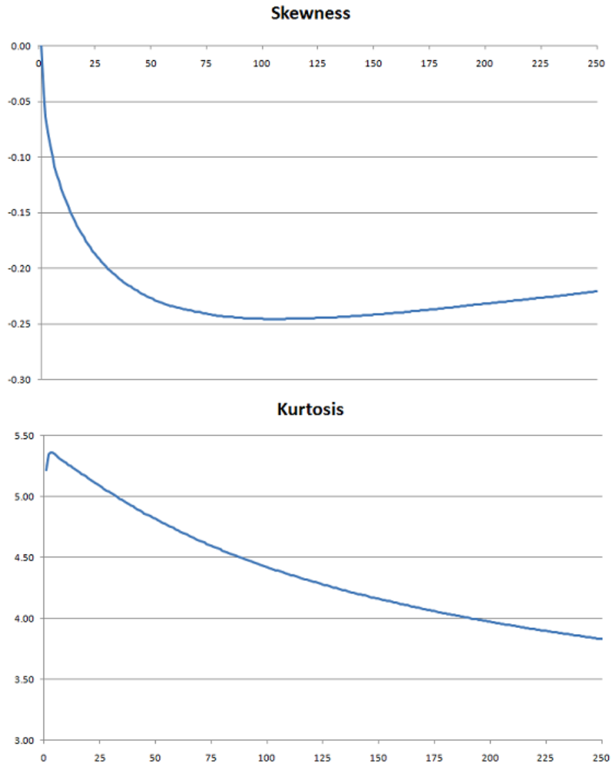
Figure 4: Skewness and kurtosis of cumulative returns from a Realized GARCH model with the log-linear specification. The x -axis gives the number of periods (days) over which returns are accumulated.
